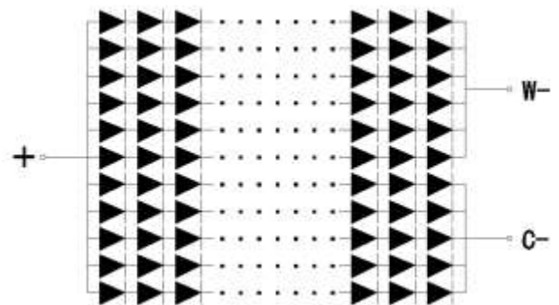
等效电路 (W:6 并 12 串 C:5 并 12 串) Equivalent-circuit (W:6parallels 12 series C:5parallels 12 series)
